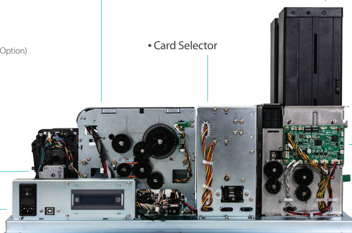
※ SMART-51DK 2 Hopper system with 300 cartridge
